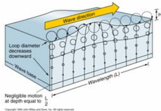
Figure 8: Water particle motion in a wave 1
